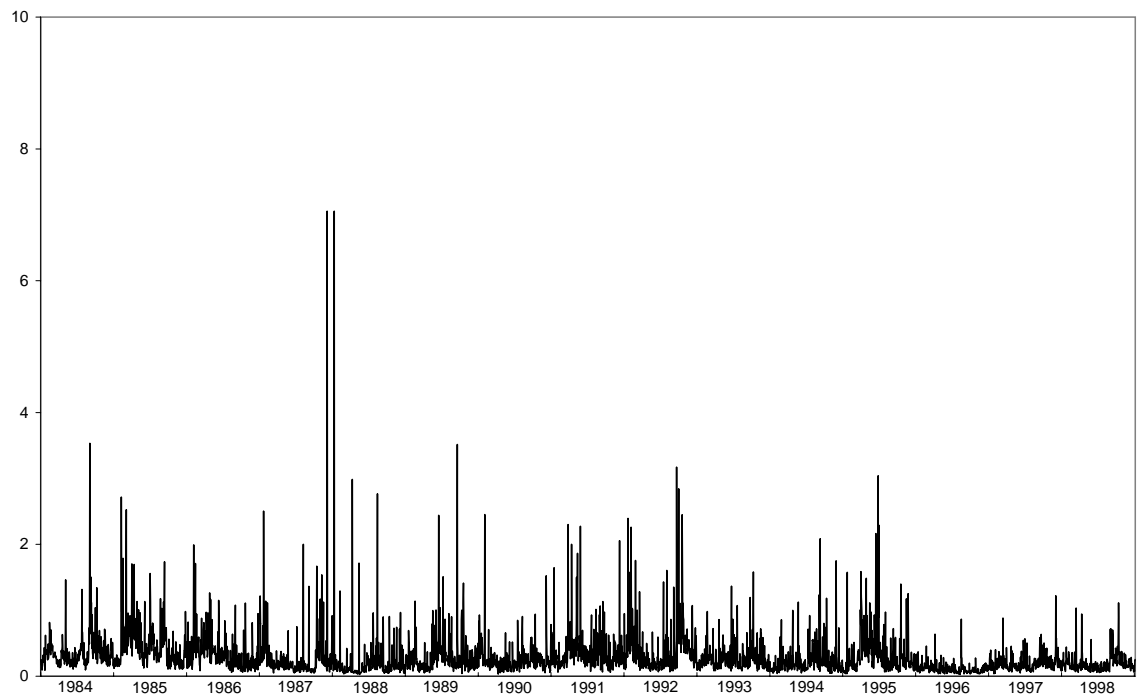
Figure 3: Daily quadratic variation computed on five-minutes log returns on the DM/$ futures contract
